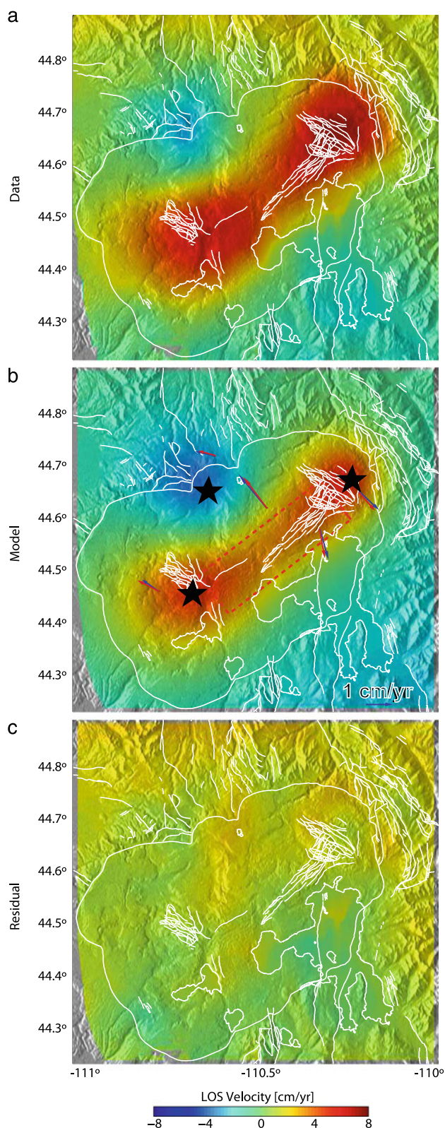
Fig. 7 The InSAR data of 2005–2006, model, and residual are represented in (a), (b), and (c), respectively. The small blue arrows in (b) represent the GPS data while the small red arrows represent the GPS model. The red rectangle in (b) is the projection of the planar source; the along-strike edge is marked with a solid red line. Projections of the Mogi sources are marked with three black stars in (b)
