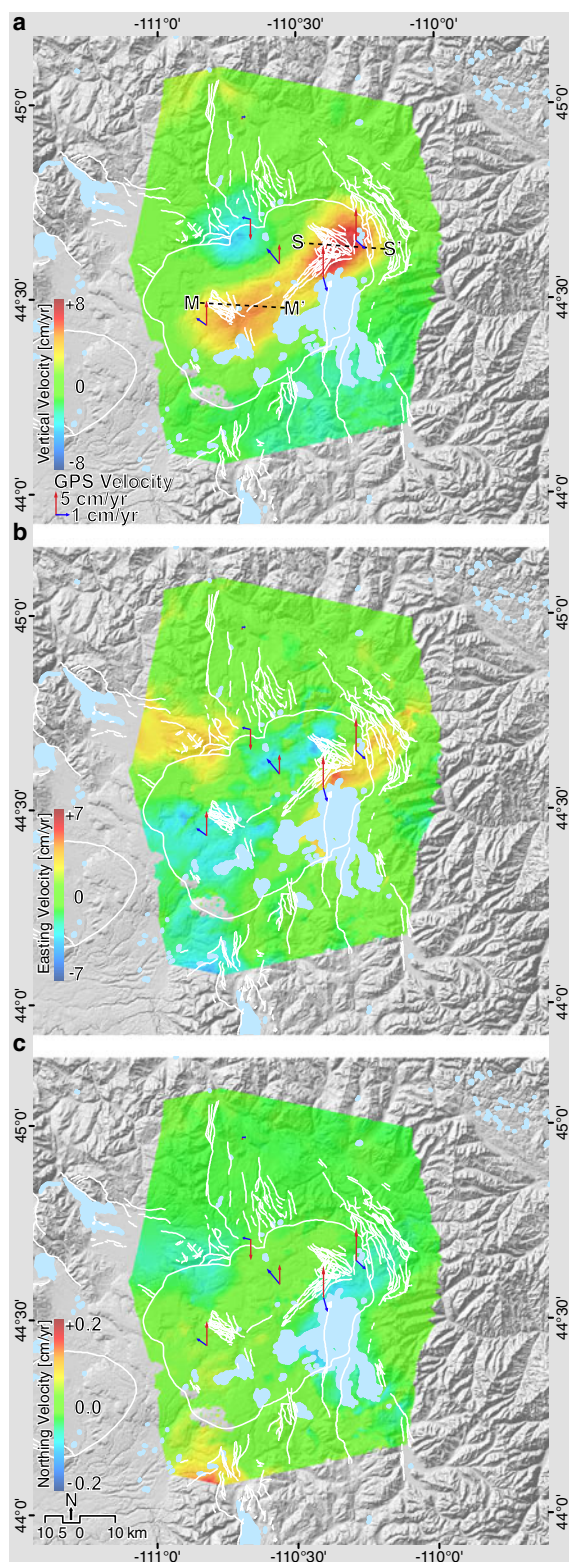
Fig. 4 InSAR three-dimensional velocity field of Yellowstone deformation between 2005 and 2006 assuming deformation results from two magma bodies underneath the Sour Creek and Mallard Lake resurgent domes. a Vertical velocity, b easting velocity, and c northing velocity. The S-S' and M-M' profiles are presented in Fig. 5a, b. The red and blue arrows indicate the vertical and horizontal GPS velocity vectors, respectively, during 2005–2006
