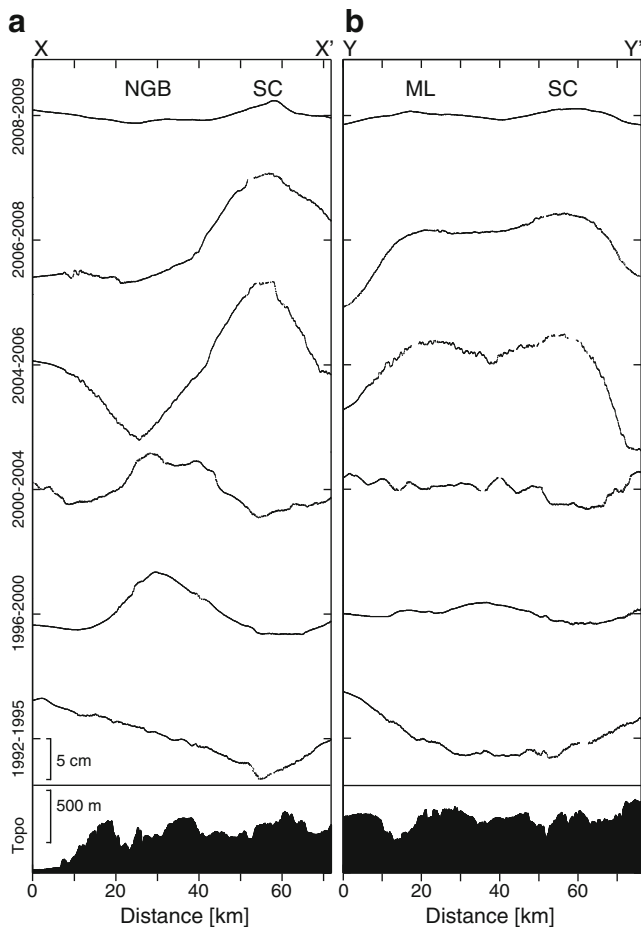
Fig. 3 Displacement profiles. a Profile X-X' through all interferograms presented in Fig. 2 and b profile Y-Y' through all interferograms presented in Fig. 2. Topography associated with the deformation profiles is shown in the bottom panels of (a) and (b) —note the topography scale starts at 2,000 m
