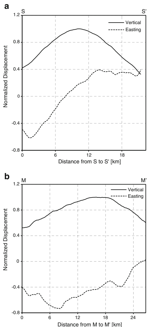
Fig. 5 Displacement profiles of the vertical and easting components. a Profile S-S' across the Sour Creek resurgent dome and b profile M-M' across the Mallard Lake resurgent dome. Values in both profiles are normalized by the maximum vertical displacement and three lines are averaged to smooth each profile. Locations of the S-S' and M-M' profiles are marked with dashed black lines in Fig. 4a
