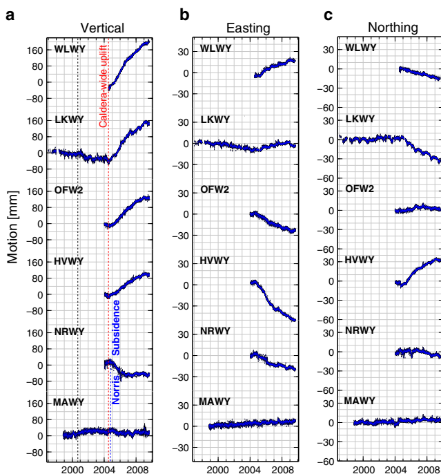
Fig. 6 GPS time series showing the three-component velocities of six continuous GPS stations (OFW2, WLWY, HVWY, NRWY, LKWY, and MAWY). Geographic locations of the GPS stations are marked with small blue triangles in Fig. 1. a Vertical motion, b easting motion, and c northing motion. This figure has been created using the Generic Mapping Tools (Wessel and Smith 1995)
