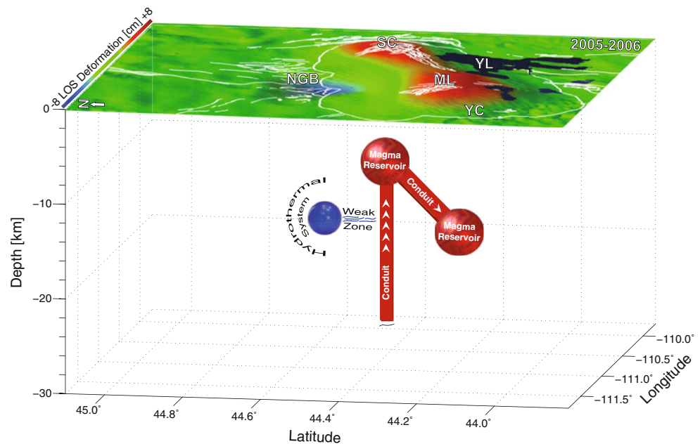
Fig. 8 Conceptual model for the Yellowstone deformation. The white lines , on the surface displacement map at the top of the model, represent the Quaternary faults and the black areas are water bodies. YL indicates Yellowstone Lake, SC Sour Creek resurgent dome, ML Mallard Lake resurgent dome, YC Yellowstone caldera, NGB Norris Geyser Basin
